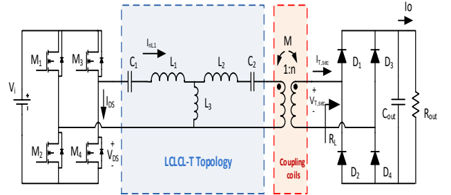
Fig. 2. LCLCL-T compensated WPT system for EV charging.
