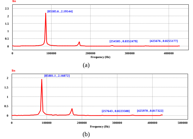
Fig. 6. PSIM simulation results of I_{in} harmonic under different \beta . (a) \beta = 0.14 . (b) \beta = 0.33 .
