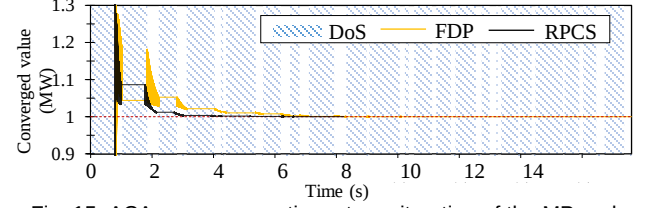
Fig. 15. ACA convergence time at one iteration of the MP under alternative DoS attack on NMGs. For the sake of clear representation, convergence of iteration value of one MG has been shown.
