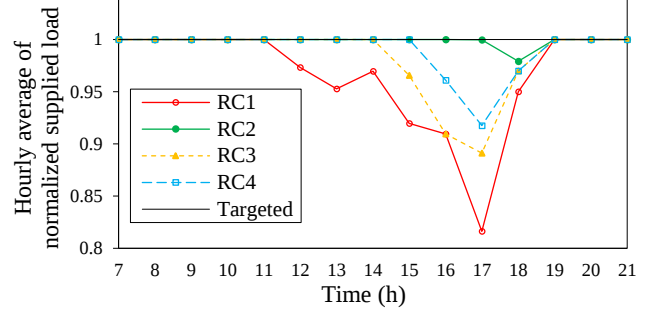
Fig. 12. Resilience curve of MG B.2 in different cases.
