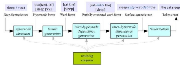
Figure 22. Workflow of the Data-Driven Generator [98].
