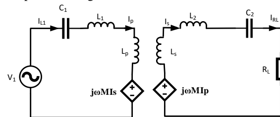
Fig. 3. Equivalent analytical circuit of the LCLCL-T topology.
